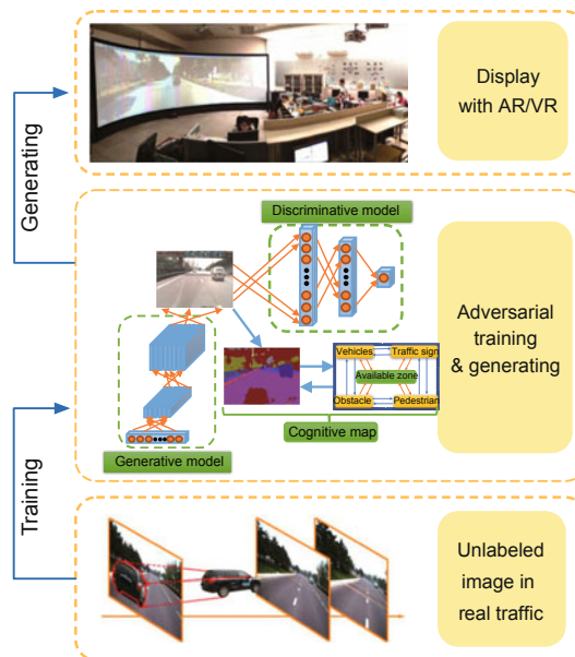
Fig. 18 Generative adversarial networks in self-driving cars
